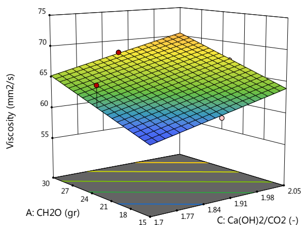
Figure 3. Impact of \text{CH}_2\text{O} mass and \text{Ca(OH)}_2/\text{CO}_2 mole ratio on kinematic viscosity (B = 7 g and D = 82.5 °C)
