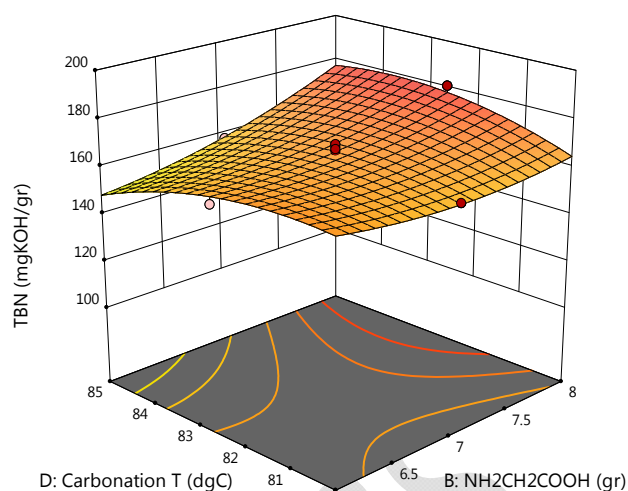
Figure 5. Impact of carbonation stage temperature and \text{NH}_2\text{CH}_2\text{COOH} mass on TBN (A = 22.5 g and C = 1.875 mol/mol)
