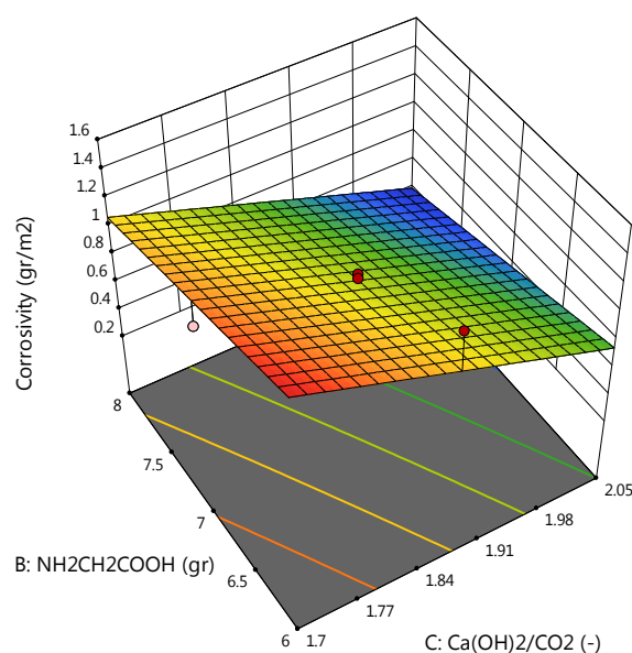
Figure 6. Impact of \text{NH}_2\text{CH}_2\text{COOH} mass and \text{Ca(OH)}_2/\text{CO}_2 mole ratio on corrosivity (A = 22.5 g and D = 82.5 °C)
